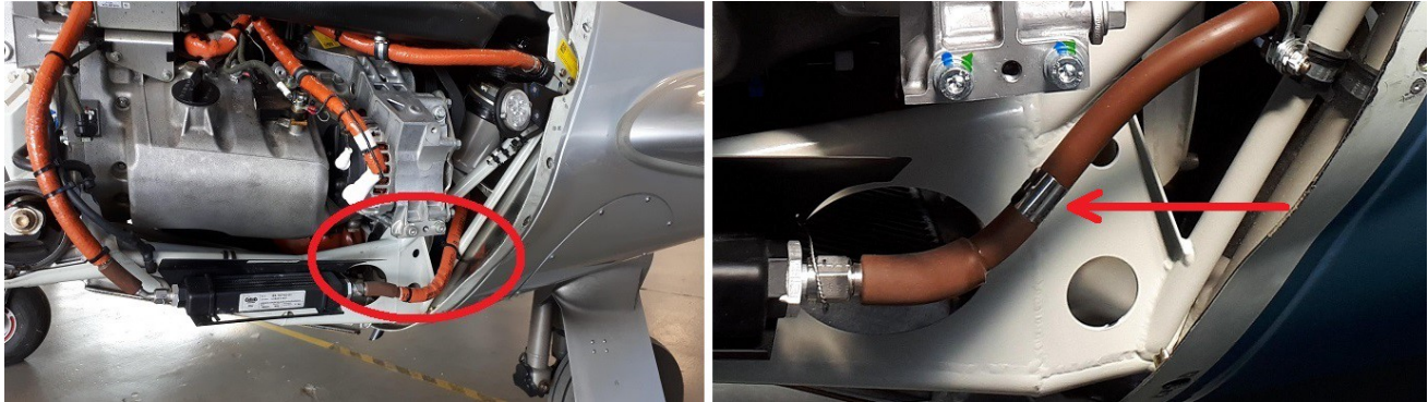
Figure 1: Left - location of fuel hose. Note the orange protective sleeve around the hose. Right - fuel hose without protective sleeve, see metallic band for the hose's part number.
