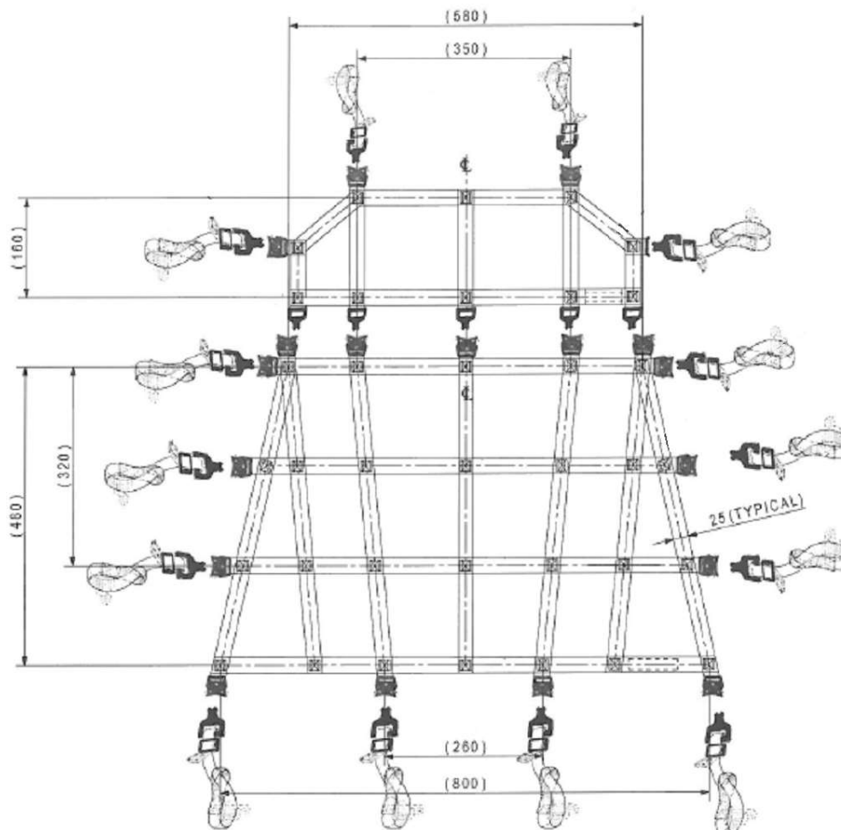
Figure 1 - DA 62 baggage net installation.
