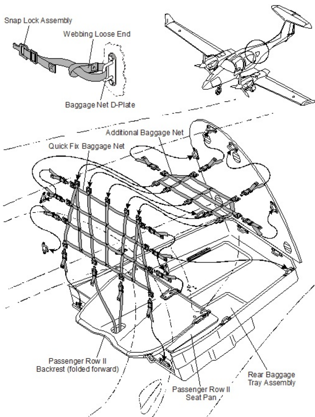
Figure 4: Rear Baggage Compartment IV (if OÄM 62-019 is carried out)
