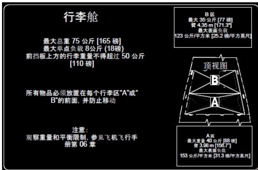
Figure 2 - Placard Baggage Compartment A and B (China Version)
