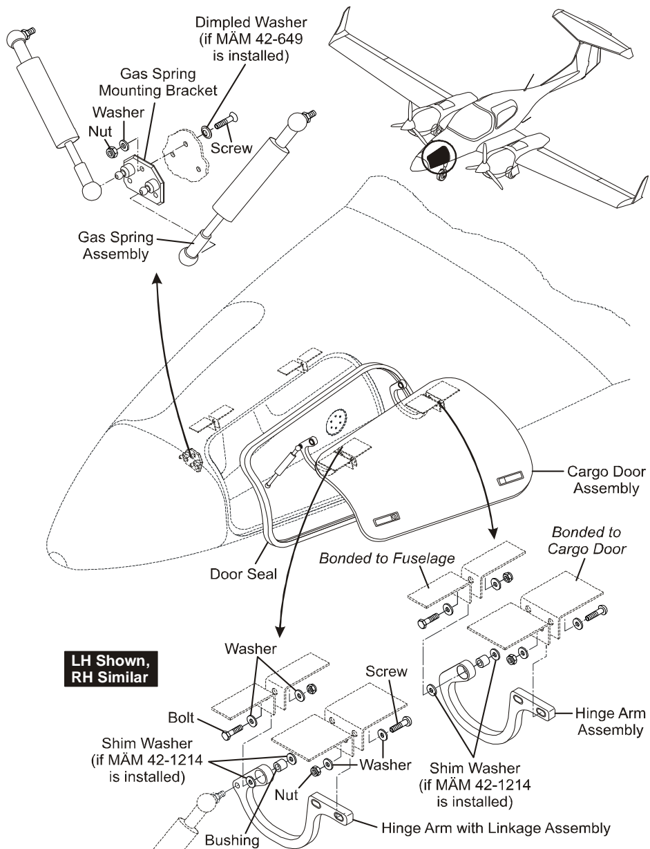
Figure 2: Front Baggage Compartment Access Doors (if MÄM 42-600 is installed)
