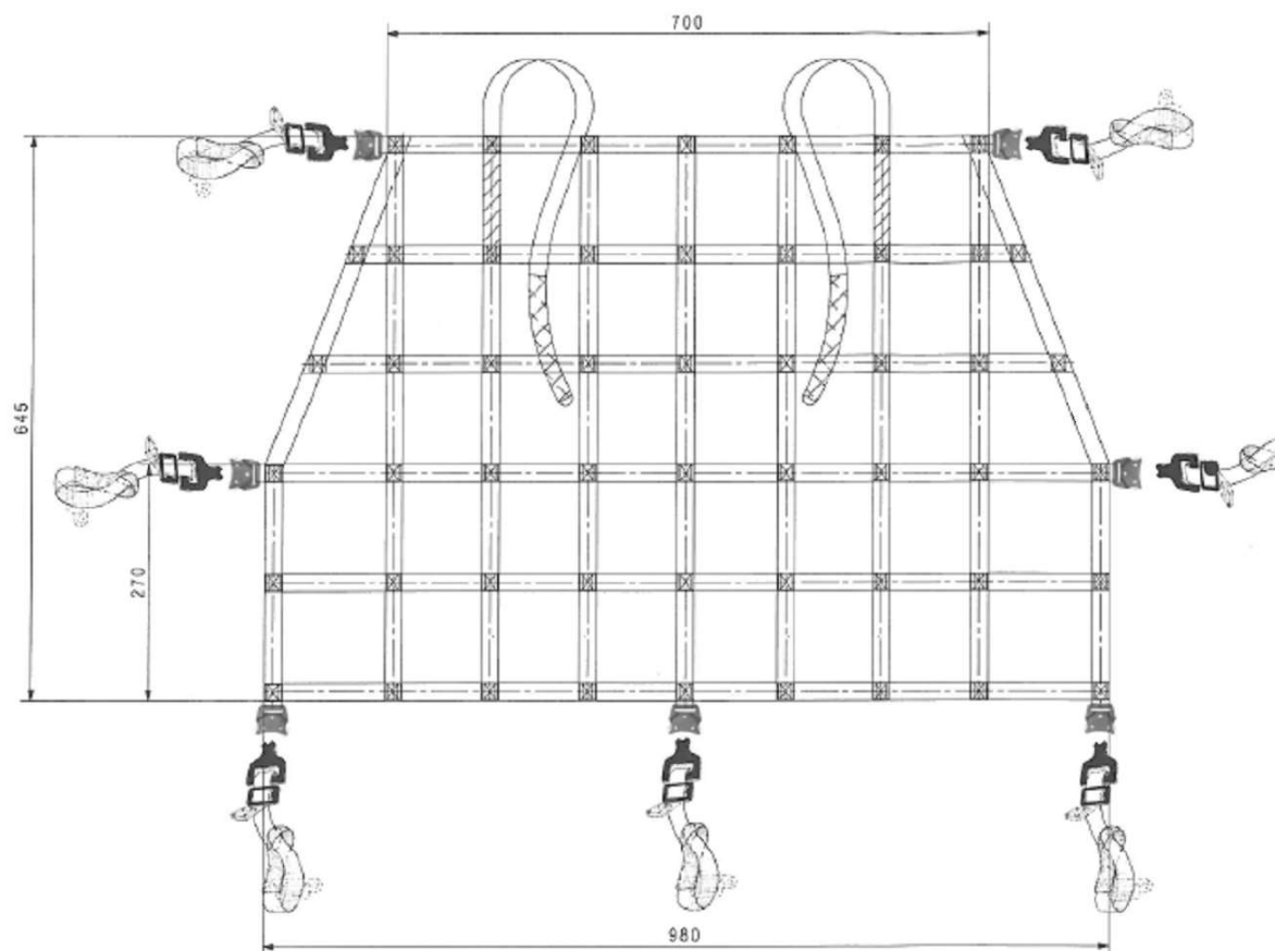
Figure 1 - Baggage net installation.
